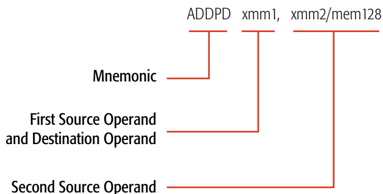
Figure 2-16. Syntax for Typical Two-Operand Instruction
