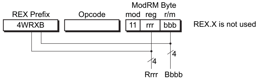
Case 1: Register-Register Addressing (No Memory Operand)
