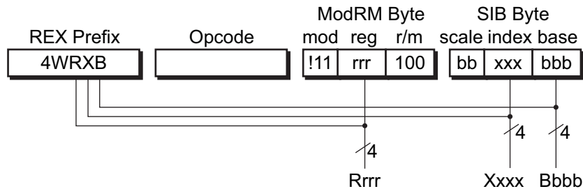
Case 3: Memory Addressing With an SIB Byte
