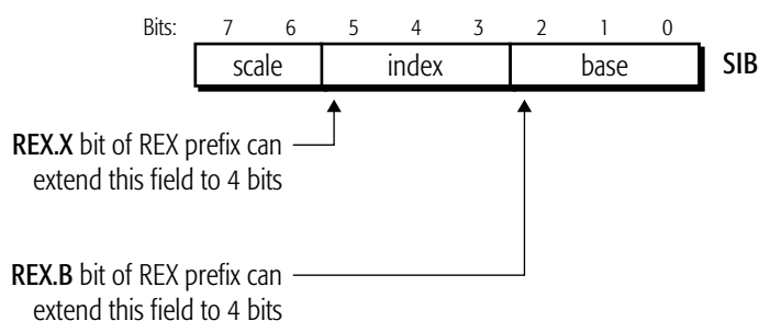
Figure 1-5. SIB Byte Format
