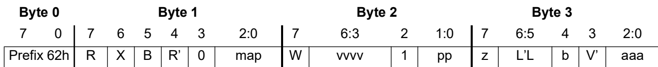
Figure 1-9. EVEX Four-byte Escape Sequence Format
