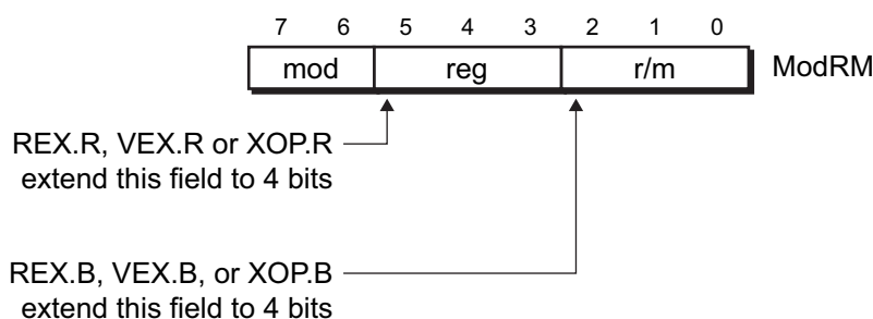
Figure 1-4. ModRM-Byte Format
