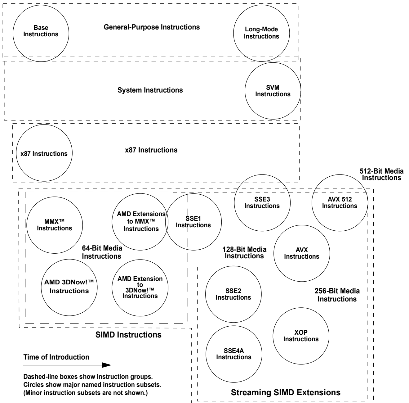
Figure D-1. AMD64 ISA Instruction Subsets
