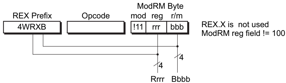
Case 2: Memory Addressing Without an SIB Byte
