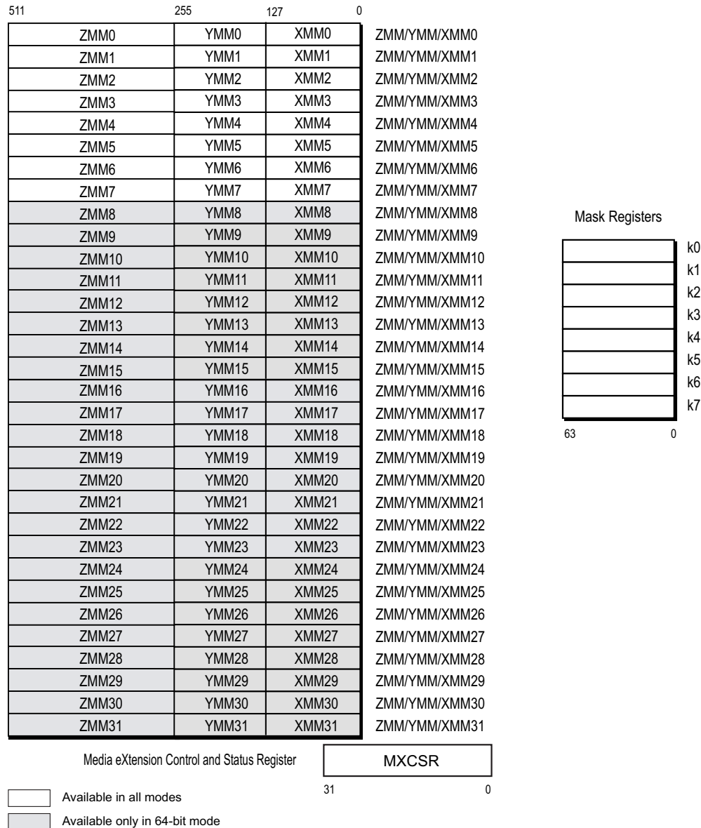
Figure 2-8. SSE Registers
