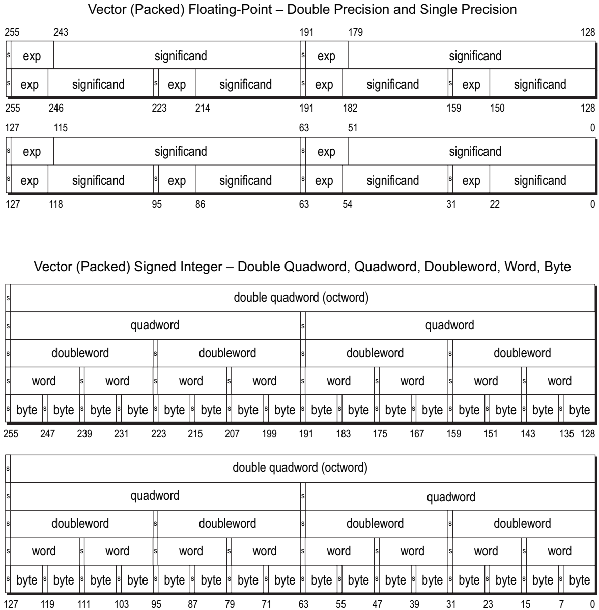
Figure 2-10. SSE 256-bit Data Types
