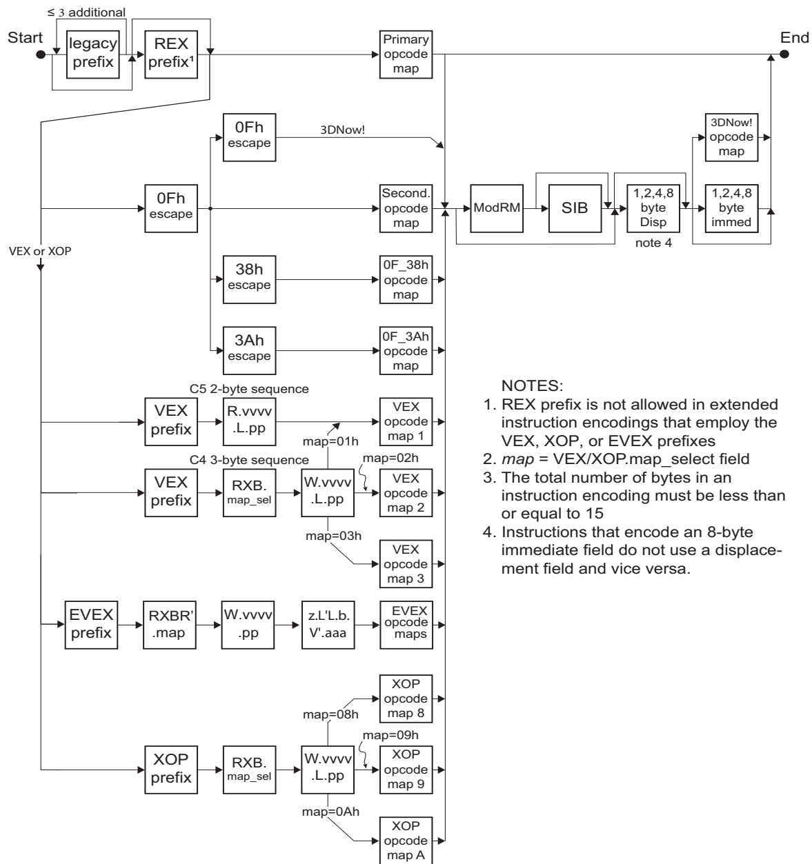
Figure 1-1. Instruction Encoding Syntax
